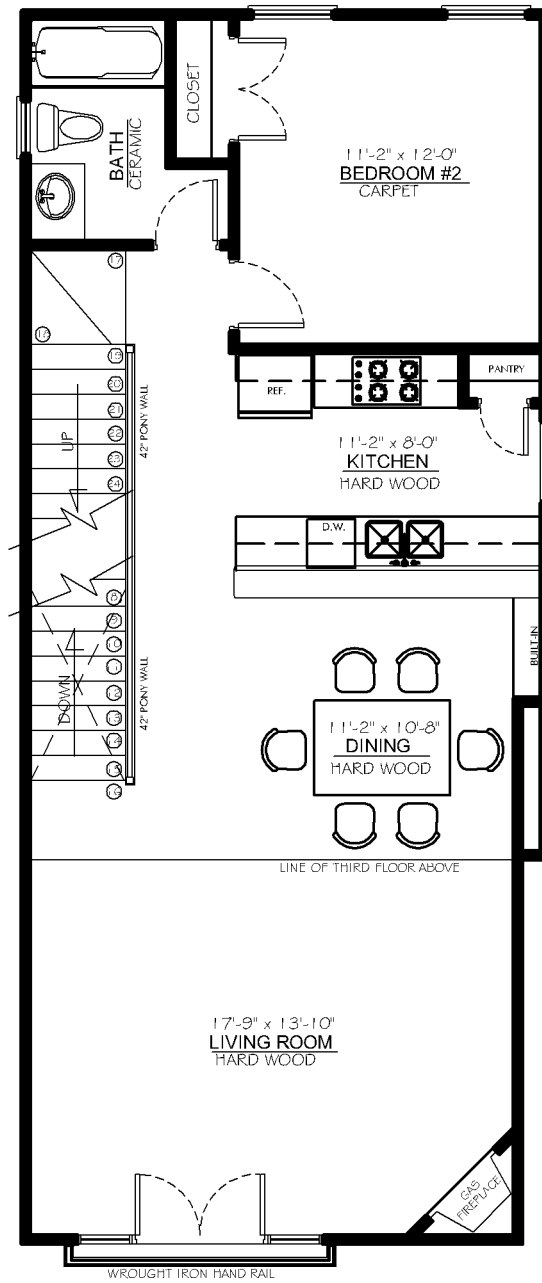
SECOND FLOOR 870 S.F.
